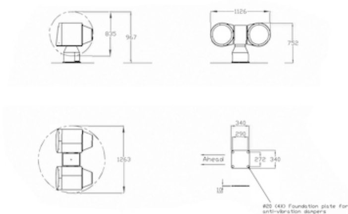
Measurement Drawing for CL35/CL35-IR and CL38/CL38-IR
